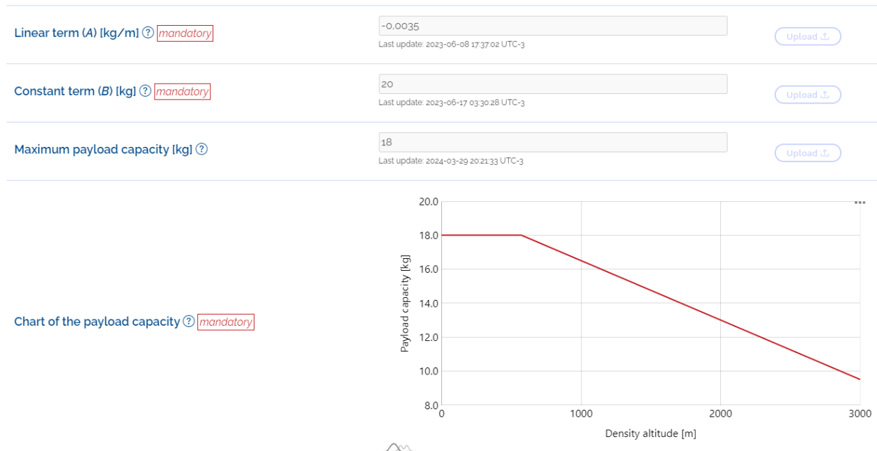
Figura 11.4: Example of Payload Capacity Estimate Graph.
